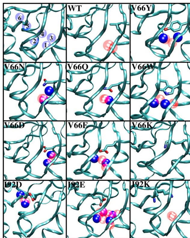
FIGURE 2 Locations of internal water molecules observed in crystallographic structures ( blue ), or MD simulations ( red ) started from the crystal hydration states. Only water molecules that have residence times longer than 1 ns are shown. Only the results of a single MD simulation for each variant are represented in this figure.
